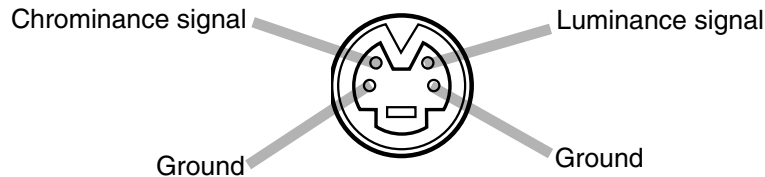
S VIDEO input (Mini DIN4 pin)
